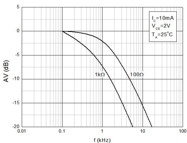
Fig.11 Frequency Response
